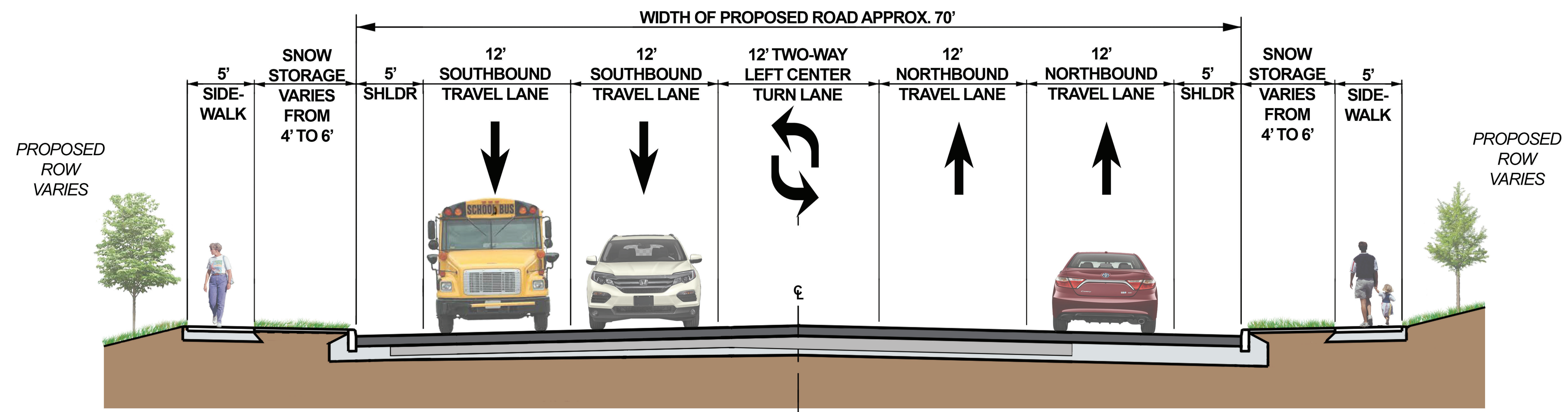
PROPOSED LANE CONFIGURATION
