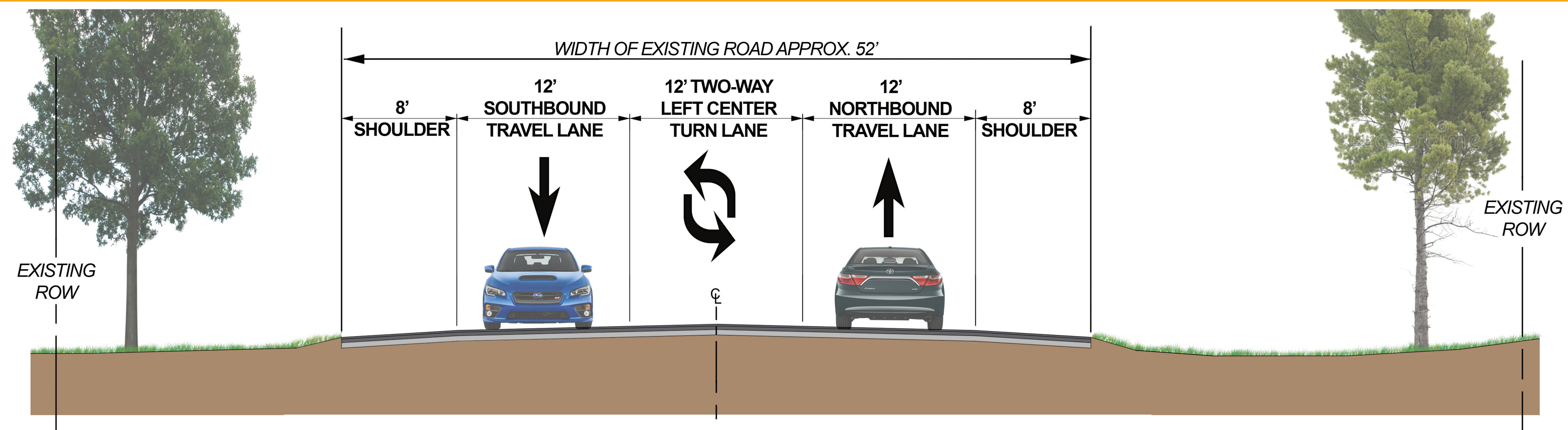
EXISTING LANE CONFIGURATION
